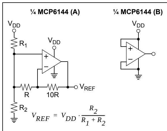
FIGURE 4-8: Unused Op Amps.
